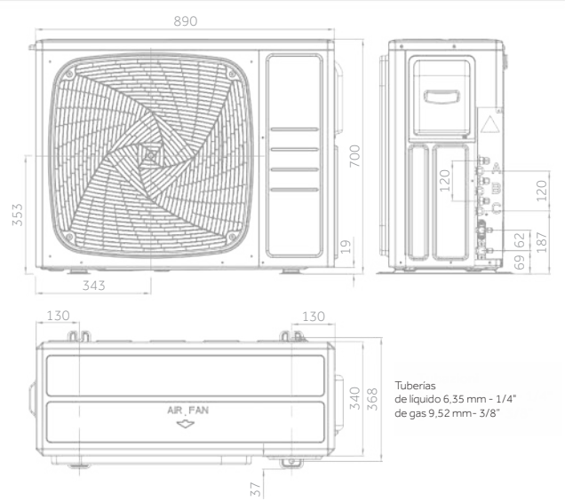
3U55S2SR5FA - 3U70S2SR5FA (3 conexiones)
